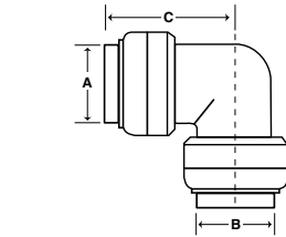
Elbow Dimensions
