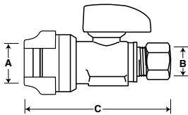
Straight Stop (Chrome Plated) Dimensions
