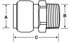
Connector Dimensions
