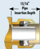
1/2" SharkBite End
