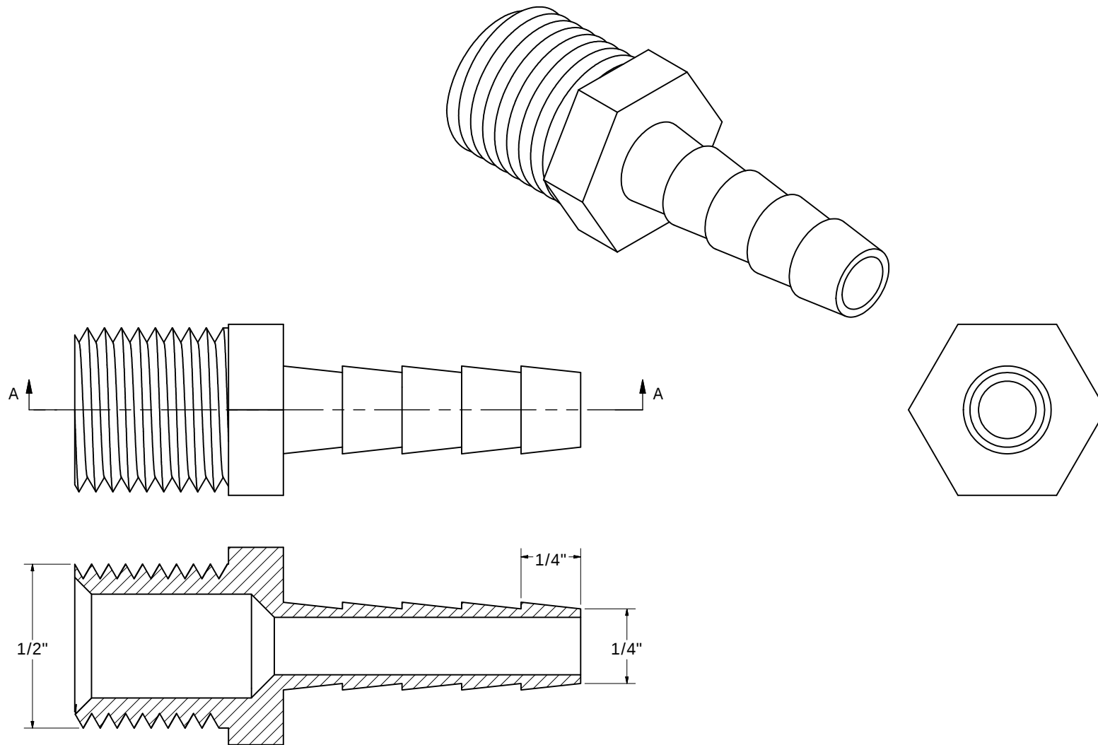
SECTION A-A SCALE 4.5
