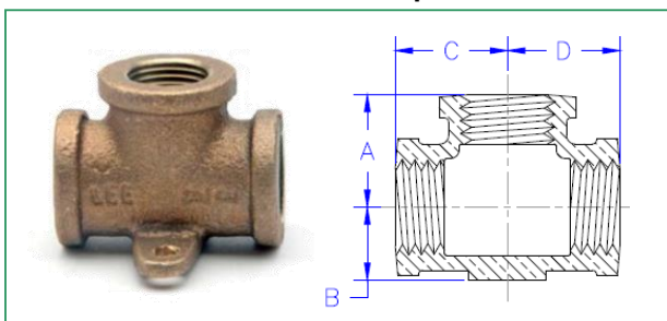
Lead Free Brass Drop Ear Tee
