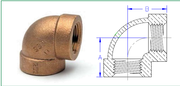
Lead Free XH Brass Elbow 90
