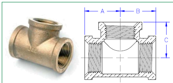
Lead Free Brass Tee
