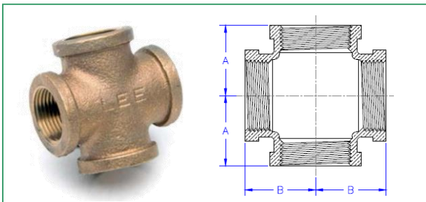
Lead Free Brass Cross
