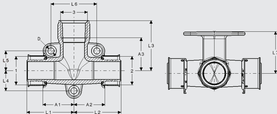
PEX Press Fire Sprinkler Vertical Tees
