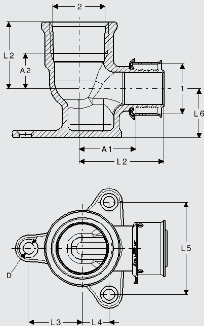
PEX Press Drop Ear Elbows
