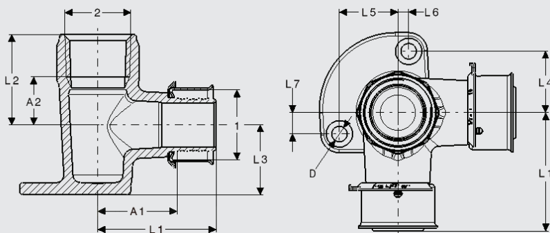
PEX Press Fire Sprinkler Elbow (Double)
