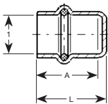
Copper Cap P - Model 2956
