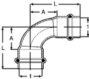
Copper 90° Elbow P x P - Model 0616
