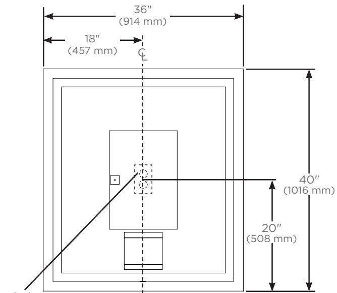
Back view for electrical outlet location
