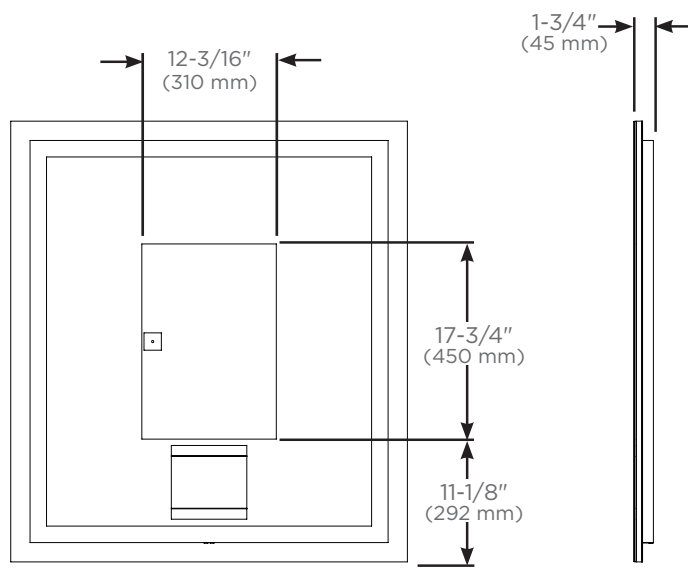
Back view for defogger location
