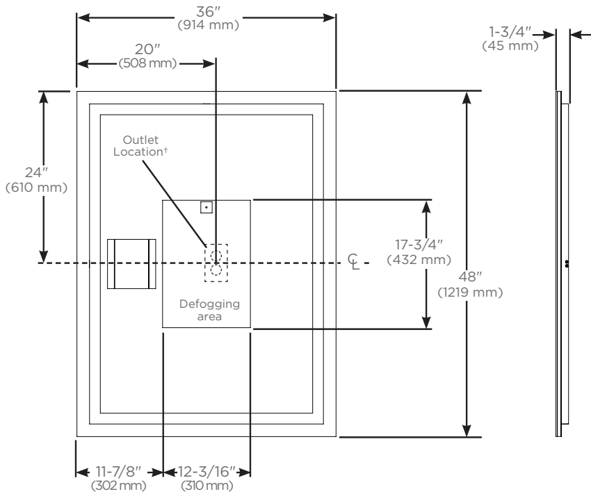
Back view for outlet and defogger location
