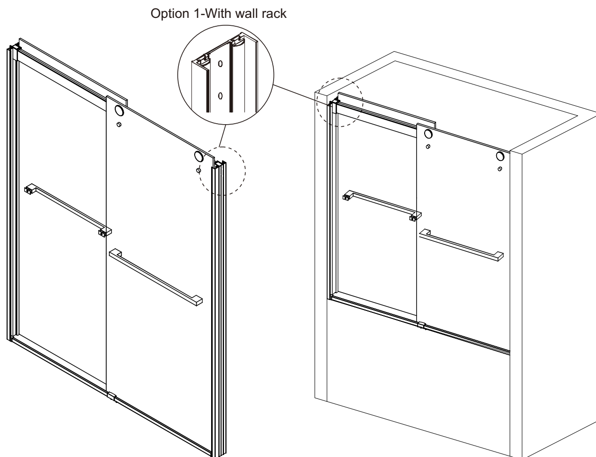
Semi-frameless shower door installation with wall rack
