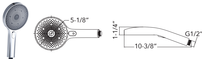
ASTRA Three Function Hand Shower SMMHSA3FR-
