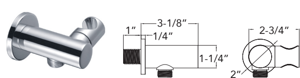
ROWAN Wall Elbow W/ Hand Shower Cradle SMRWEH-
