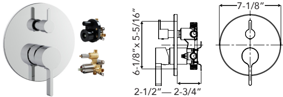
THEO Two Function Pressure Balance Valve SMVTP2R-
