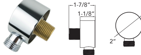
TYLER Wall Elbow SMTWE-
