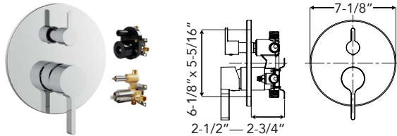
THEO Three Function Pressure Balance Valve SMVTP3R-
