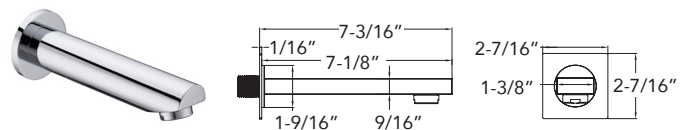
ROWAN Non-diverting Tub Spout SMRTS-
