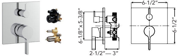
THEO Two Function Pressure Balance Valve SMVTP3S-
