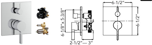
THEO Two Function Pressure Balance Valve SMVTP3S-
