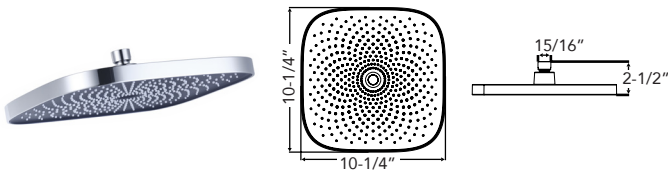
ASTRA Single Function Showerhead SMMSHA10S-
