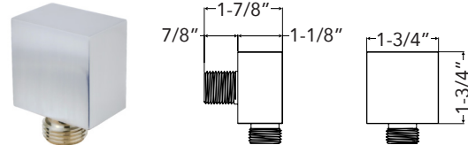
MANHATTAN Wall Elbow SMMWE-
