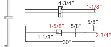
SAMPSON 30" Sliding Bar SMSSSB30-
