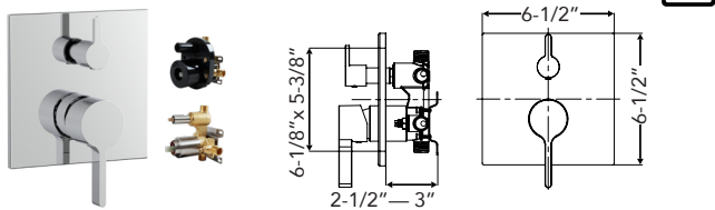
THEO Three Function Pressure Balance Valve SMVTP3S-
