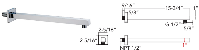
SAMPSON 16" Shower Arm SMSSA16-
