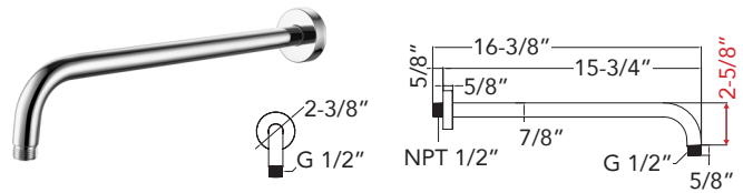
ROWAN 16" Shower Arm SMRSA16-
