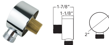
TYLER Wall Elbow SMTWE-
