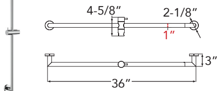
TYLER 36" Sliding Bar SMTSSB36-
