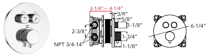
ARGOTHERM Two Function Thermostatic Valve SMVAT2R-
