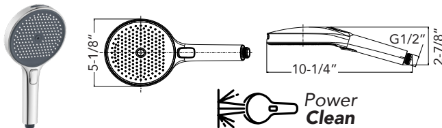
OSCAR Four Function Hand Shower SMMHSO4FR-
