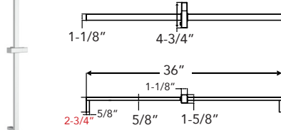
SAMPSON 36" Sliding Bar SMSSSB36-
