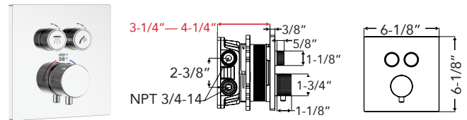
ARGOTHERM Two Function Thermostatic Valve SMVAT2S-
