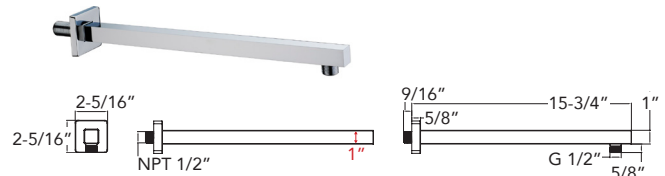
SAMPSON 16" Shower Arm SMSSA16-
