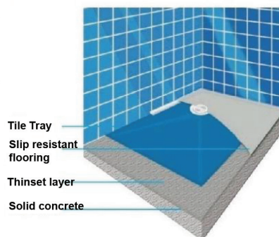
Installation with concrete floors
