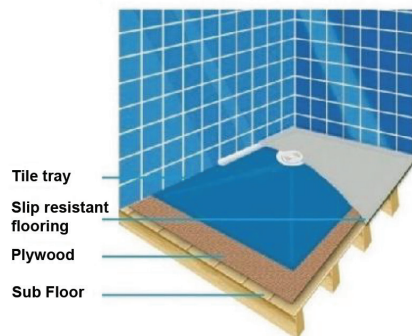
Installation with wood floors
