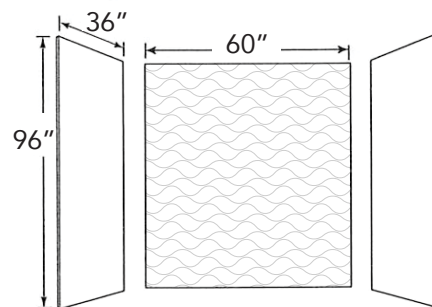
*Gali Wave Specification Drawing
