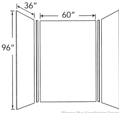
*Pioneer Plus Specification Drawing
