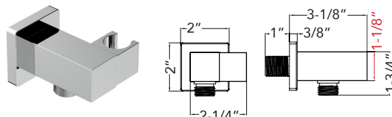
SAMPSON Wall Elbow W/ Hand Shower Cradle SMSWEH-
