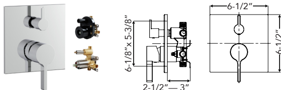
THEO Two Function Pressure Balance Valve SMVTP3S-
