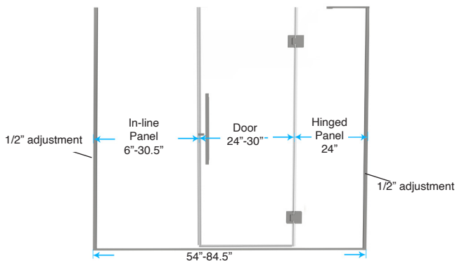
Type F Glass to Glass Hinged Door & (2) Panels w/ L Bracket
