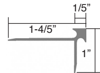
SMTTOCT Outside Corner Trim
