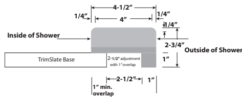
MAXIMUM DEPTH ADJUSTMENT with Add-On Threshold TrimSlate base depth + 2-1/2"
