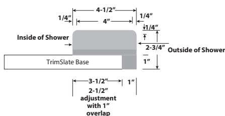
MINIMUM DEPTH ADJUSTMENT with Add-On Threshold TrimSlate base depth + 1"
