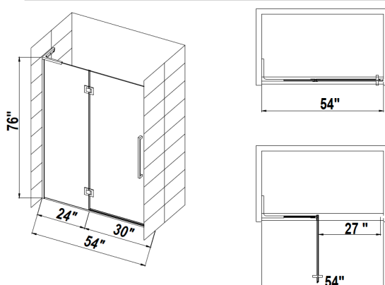
Type E 24" Fixed Hinged Panel w/ Door (Reversible L Bracket Included) Width Available 48"-54", 1" increment
