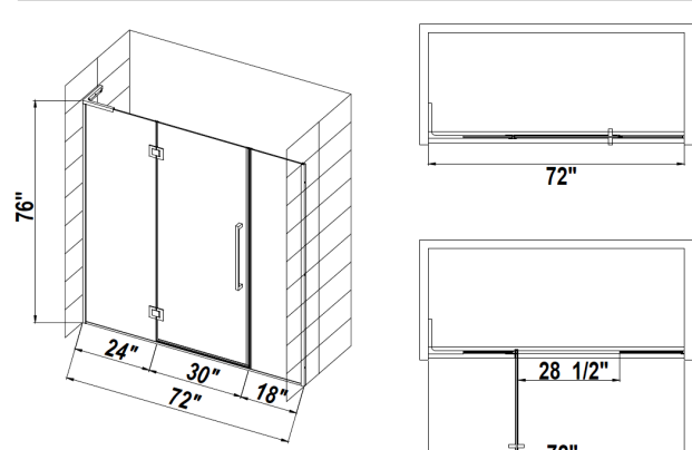
Type F 24" Fixed Hinged Panel w/ Door & In-line Panel (Reversible L Bracket Included) Width Available 54"-84.5", 1/2" increment
