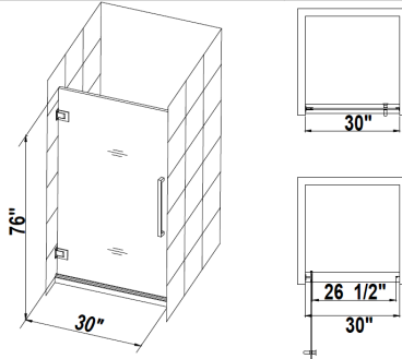
Type C 6" Fixed Hinged Panel w/ Door Width Available 30"-36", 1" increment
