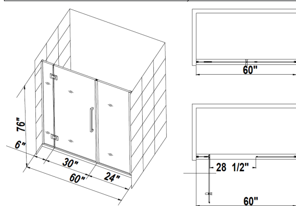
Type F 24" Fixed Hinged Panel w/ Door & In-line Panel (Reversible L Bracket Included) Width Available 54"-84.5", 1/2" increment
