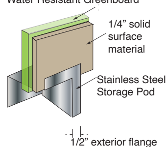
Vertical Storage Pod detail Water Resistant Greenboard
