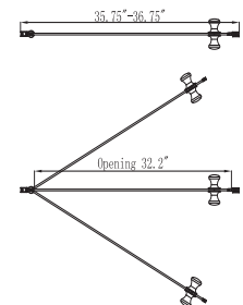
Drawing for SMLS367006C-
