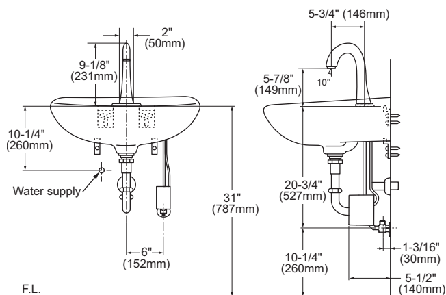
Single Supply
