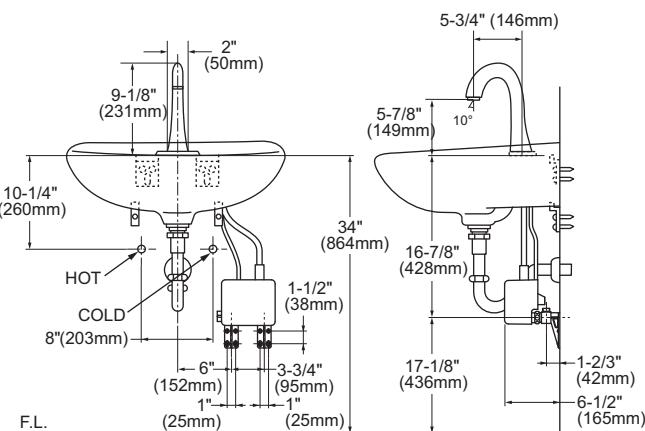
Thermal Mixing
