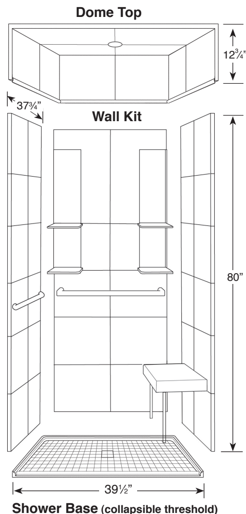
Shown with FC3938 Shower Base, T3981 Dome Top and GB1529PS Grab Bar set, GBHS18PS Hand Shower
