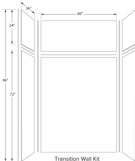
Transition Wall Kit PPWKX60367224
