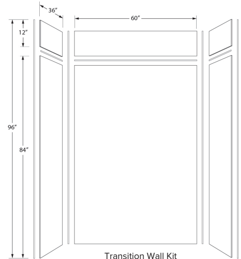
Transition Wall Kit PPWKX60368412
