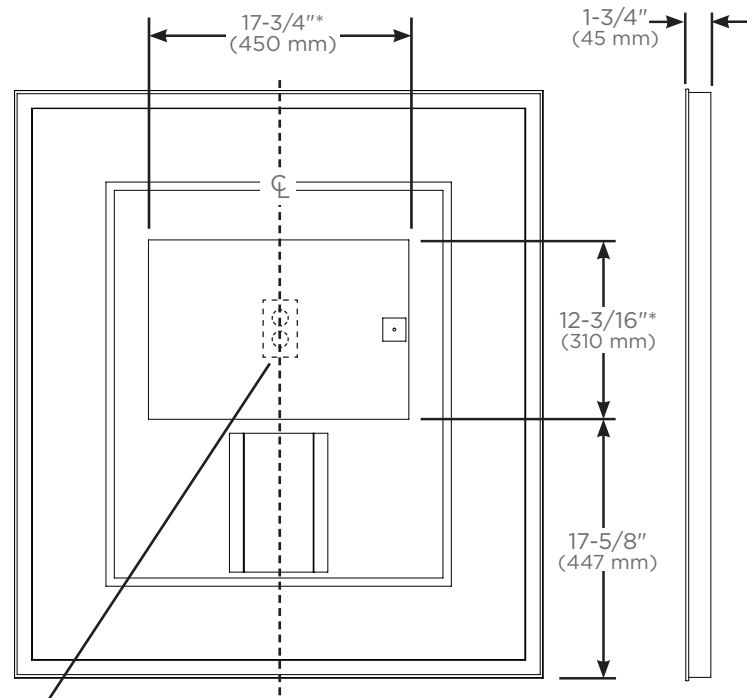
Back view for electrical outlet location
