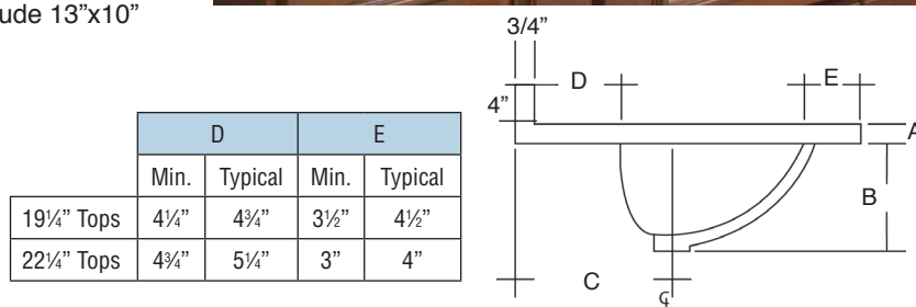
Giallo Veneziano granite vanity top with undermount china oval bowl, beveled front edge
