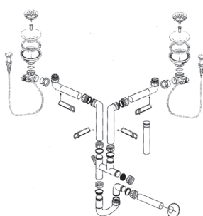
2 Remote Sink Strainers
