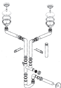
2 Sink Strainers
