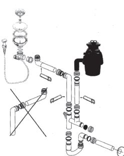
1 Sink Strainer and 1 Disposer Strainer
